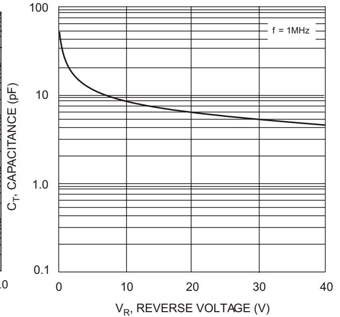
Fig. 2 Typical Total Capacitance vs Reverse Voltage
